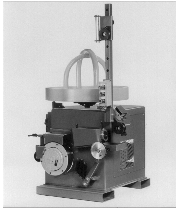
RMG Model 12 In-Line Wire Drawing Machine shown here in Spacesaver configuration.
