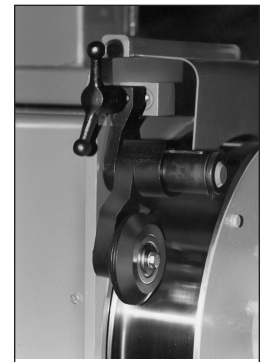
4" Manual spring-loaded Wire-Relaxer roller is standard on Model 34 and 45 wire drawers.
